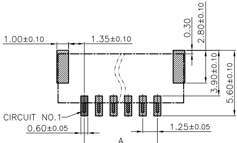
RECOMMENDED PCB. LAYOUT DEFAULT TOLERANCE:±0.10(TOP VIEW)
